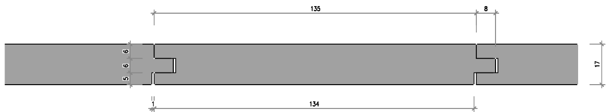
Nr. 4145-M N+K 17/135 mm, Kamm 8 mm lang parallel
